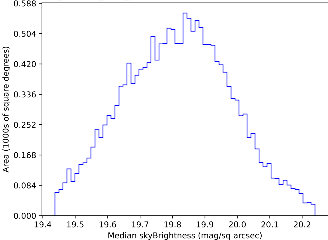
noroll_mjdp60_v3.4_10yrs WFD all bands: Median skyBrightness
