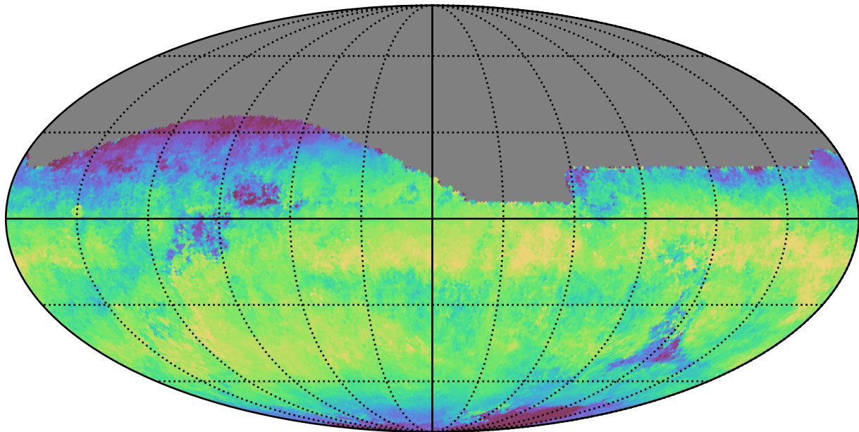
noroll_mjdp60_v3.4_10yrs All sky z band: Median skyBrightness
