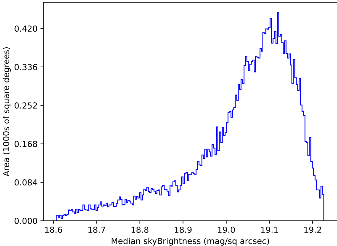
noroll_mjdp60_v3.4_10yrs All sky z band: Median skyBrightness
