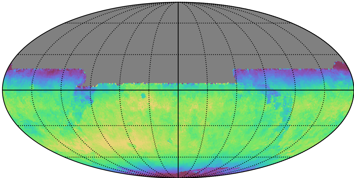
noroll_mjdp60_v3.4_10yrs All sky y band: Median skyBrightness
