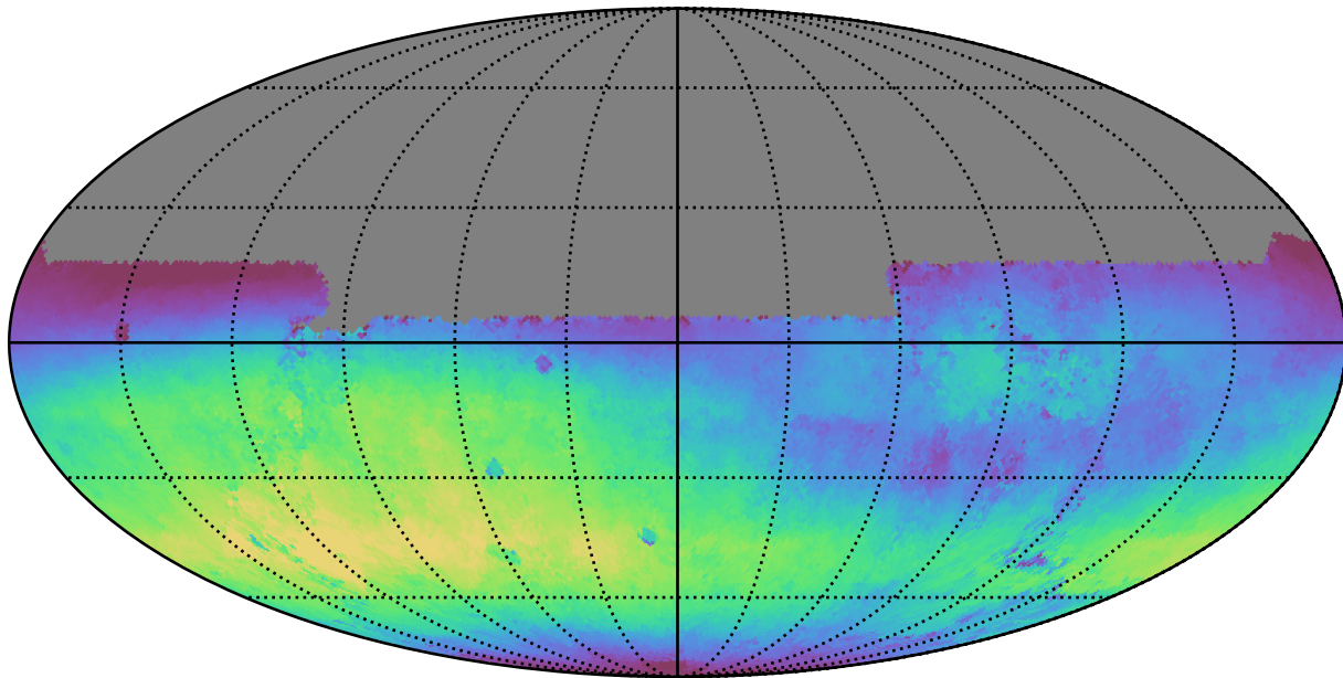
noroll_mjdp60_v3.4_10yrs All sky u band: Median skyBrightness
