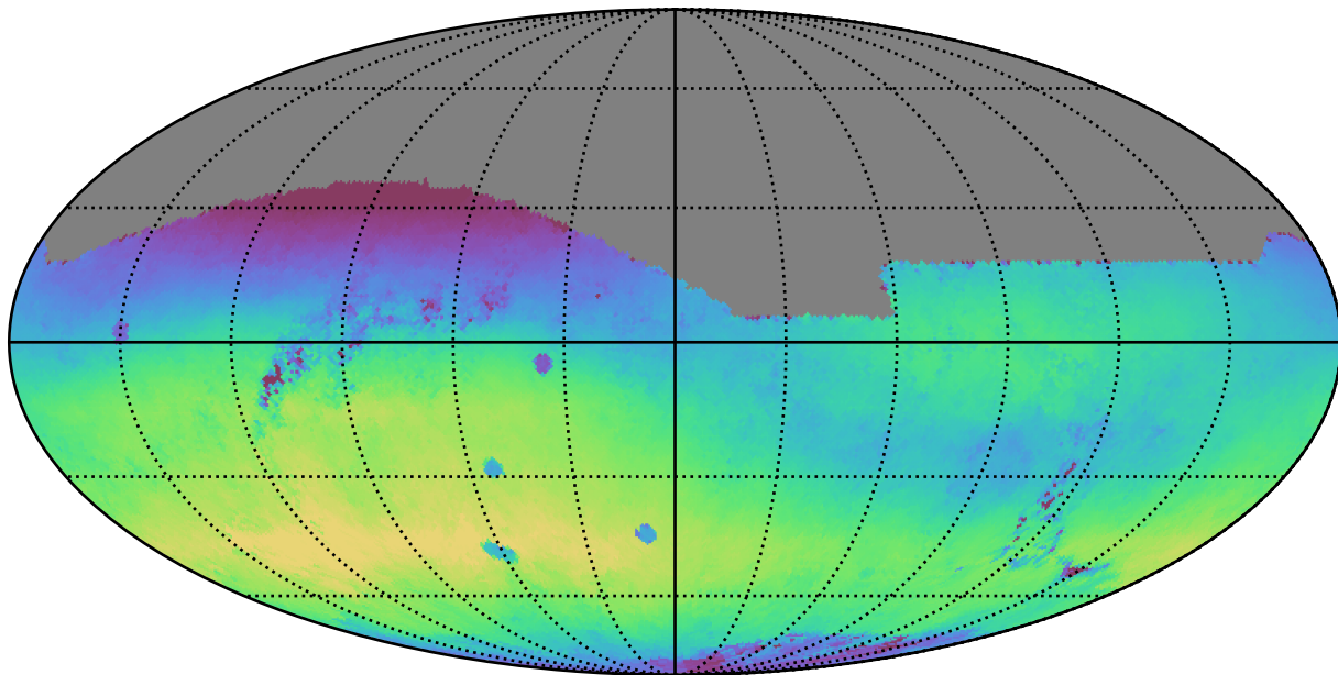
noroll_mjdp60_v3.4_10yrs All sky r band: Median skyBrightness
