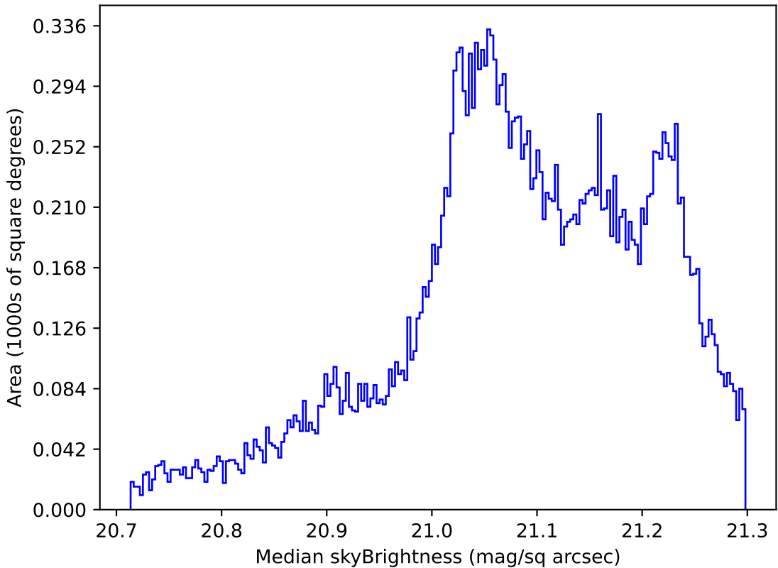
noroll_mjdp60_v3.4_10yrs All sky r band: Median skyBrightness
