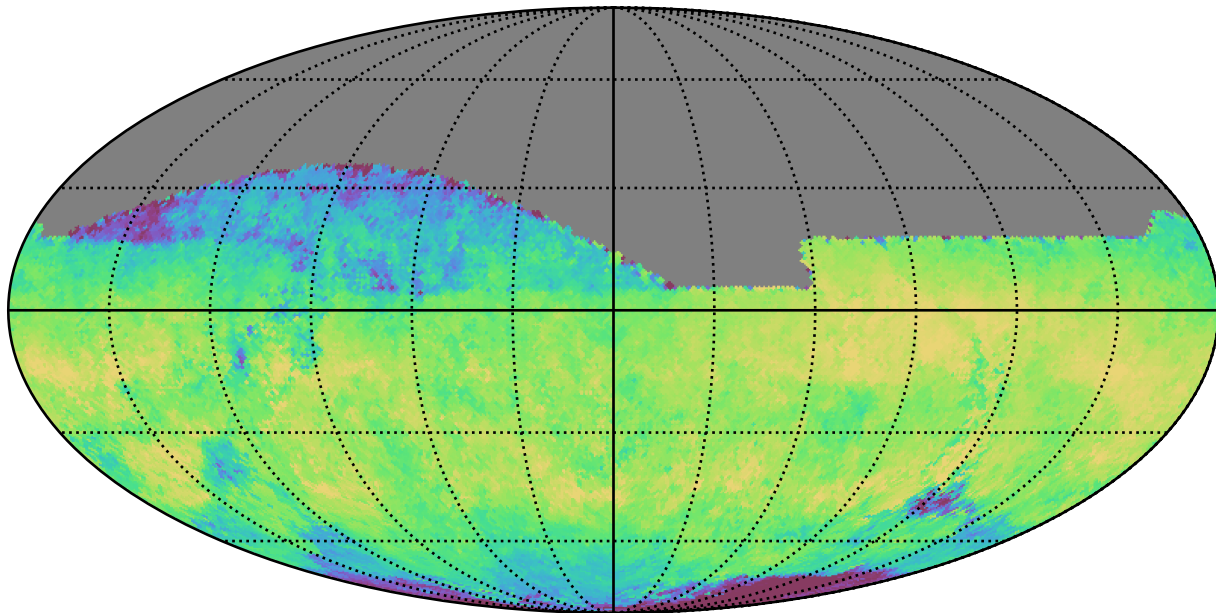
noroll_mjdp60_v3.4_10yrs All sky i band: Median skyBrightness
