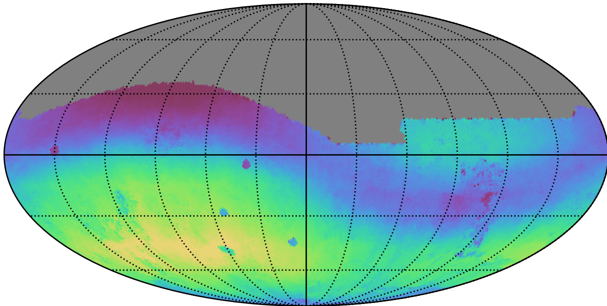
noroll_mjdp60_v3.4_10yrs All sky g band: Median skyBrightness
