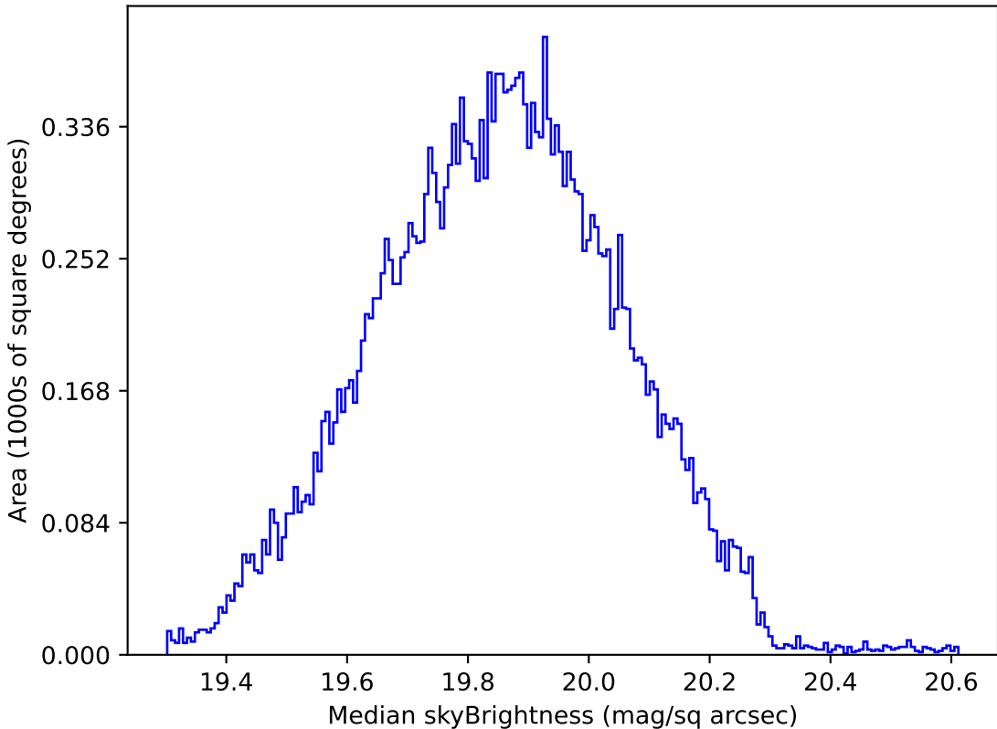
noroll_mjdp60_v3.4_10yrs All sky all bands: Median skyBrightness
