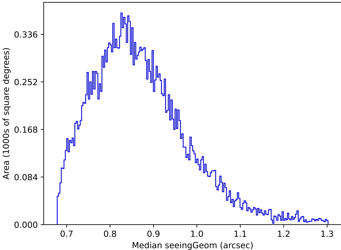
noroll_mjdp60_v3.4_10yrs Yr 1 z band: Median seeingGeom
