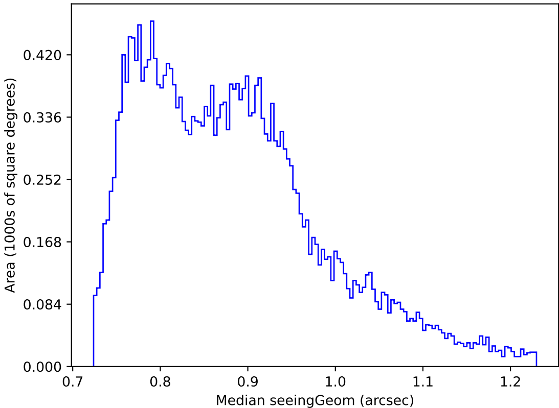
noroll_mjdp60_v3.4_10yrs Yr 1 all bands: Median seeingGeom
