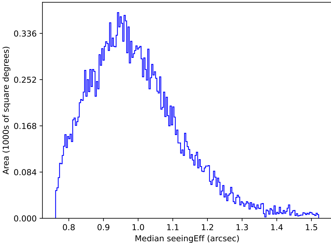
noroll_mjdp60_v3.4_10yrs Yr 1 z band: Median seeingEff
