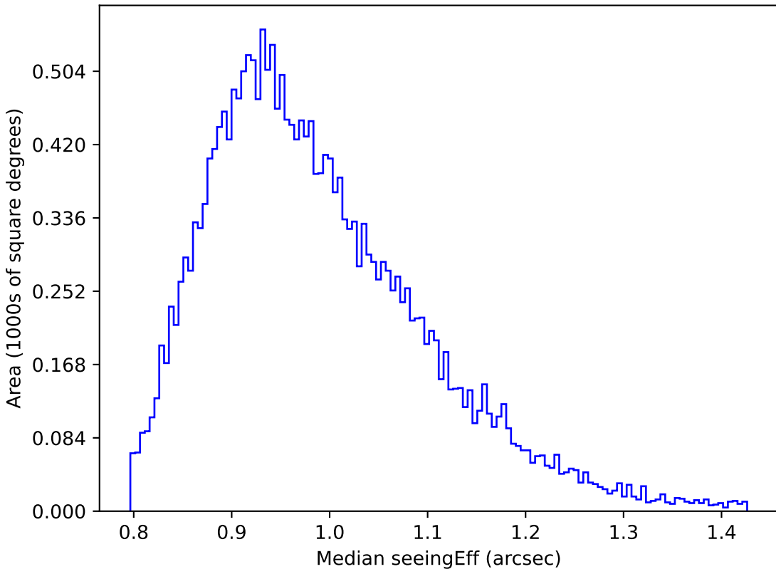
noroll_mjdp60_v3.4_10yrs Yr 1 y band: Median seeingEff
