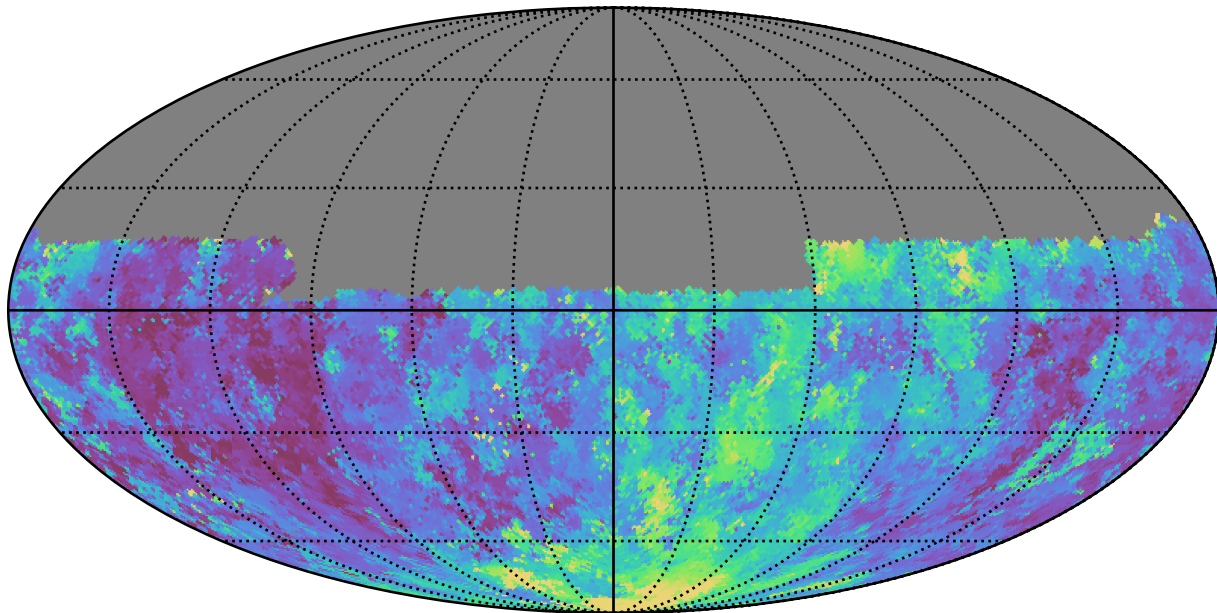
noroll_mjdp60_v3.4_10yrs Yr 1 u band: Median seeingEff
