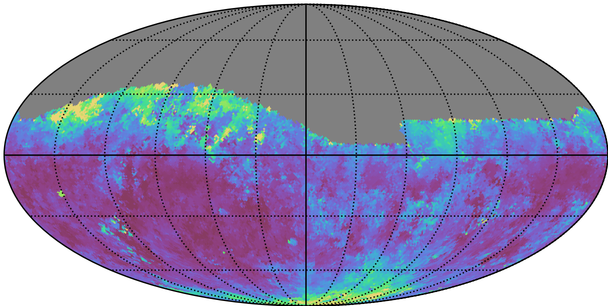
noroll_mjdp60_v3.4_10yrs Yr 1 i band: Median seeingEff
