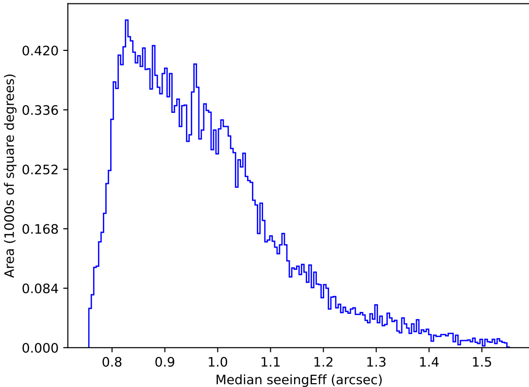
noroll_mjdp60_v3.4_10yrs Yr 1 i band: Median seeingEff
