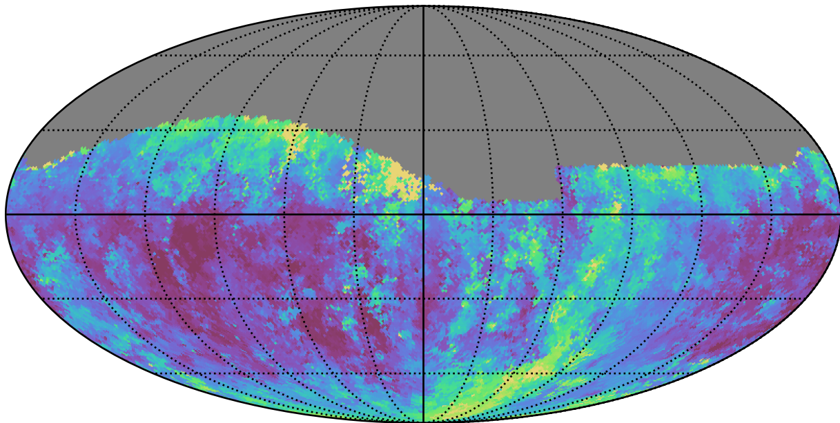
noroll_mjdp60_v3.4_10yrs Yr 1 g band: Median seeingEff
