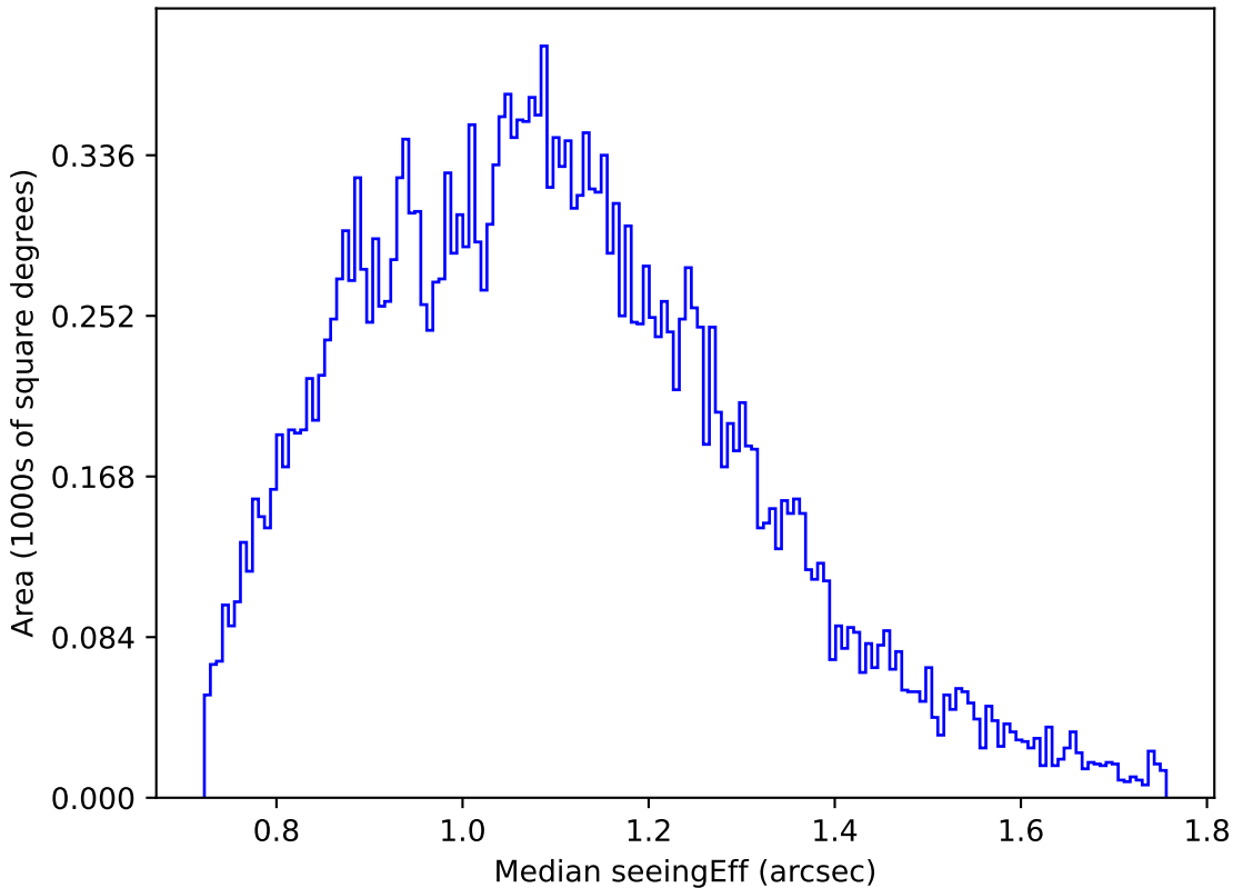
noroll_mjdp60_v3.4_10yrs Yr 1 g band: Median seeingEff
