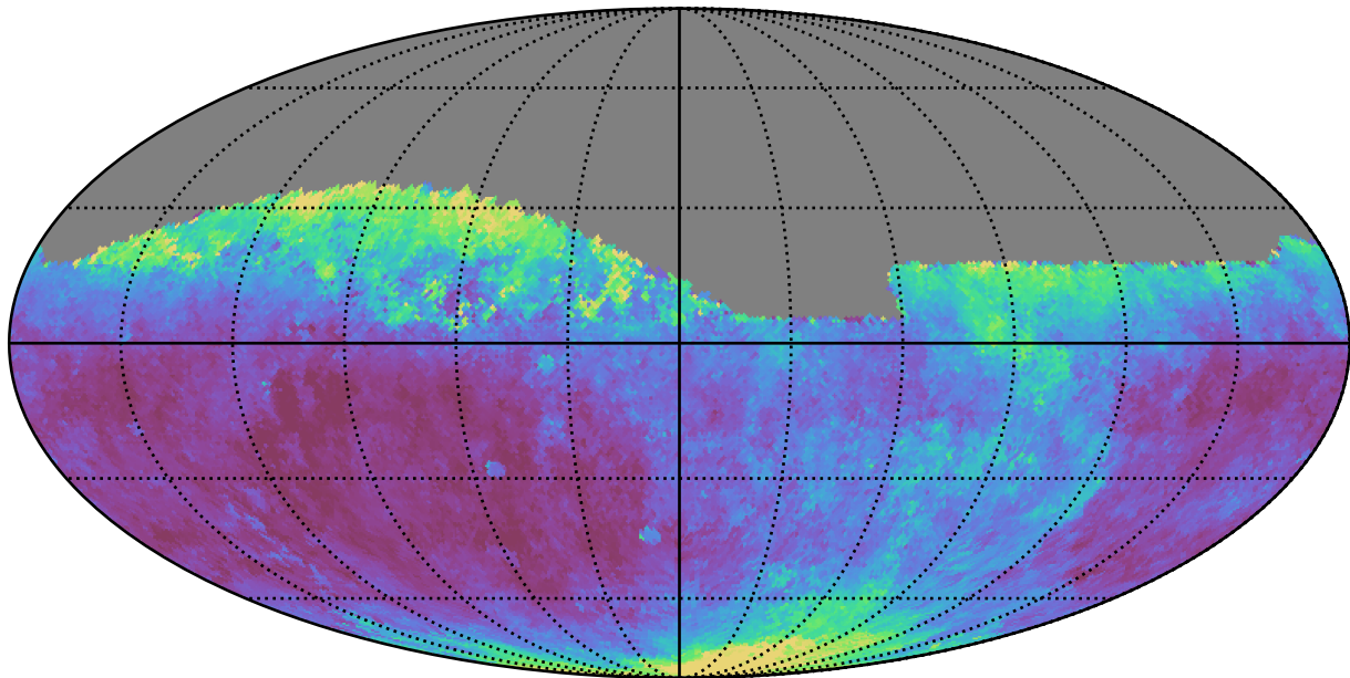
noroll_mjdp60_v3.4_10yrs Yr 1 all bands: Median seeingEff
