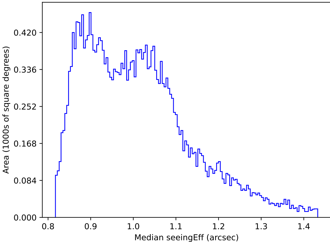
noroll_mjdp60_v3.4_10yrs Yr 1 all bands: Median seeingEff
