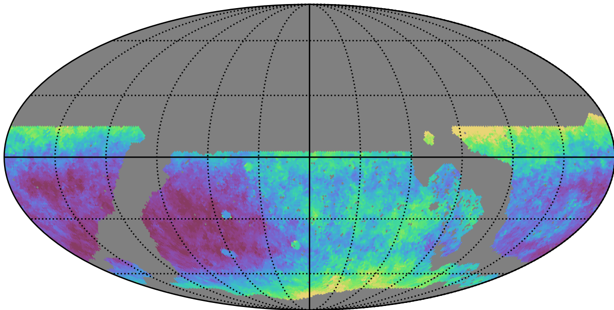
noroll_mjdp60_v3.4_10yrs WFD z band: Median seeingEff
