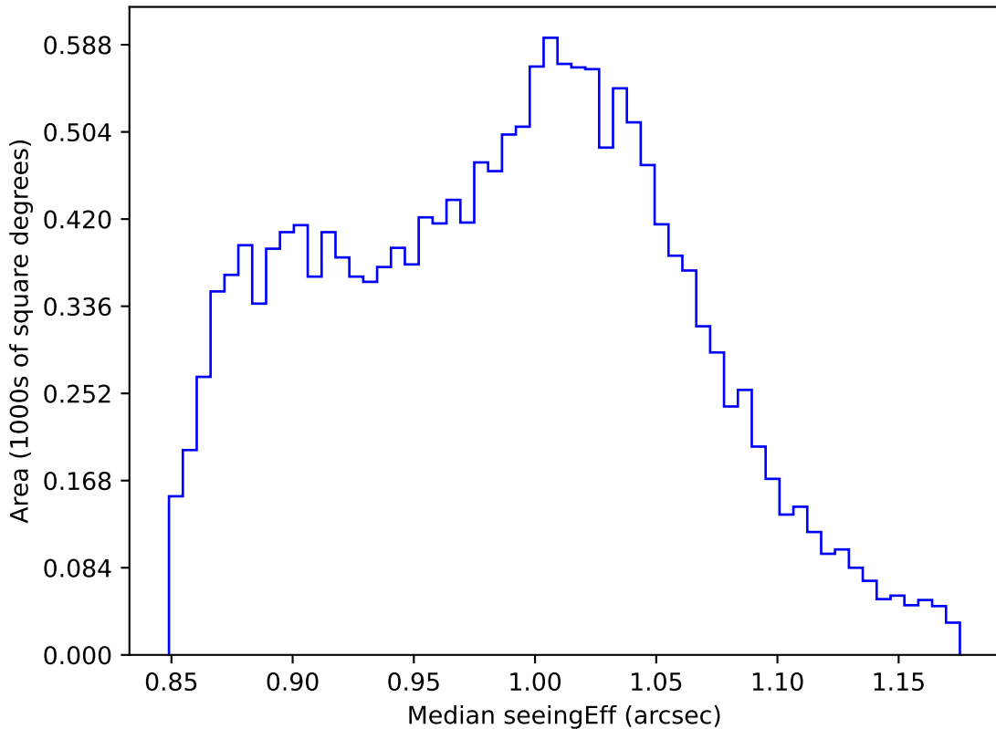
noroll_mjdp60_v3.4_10yrs WFD z band: Median seeingEff
