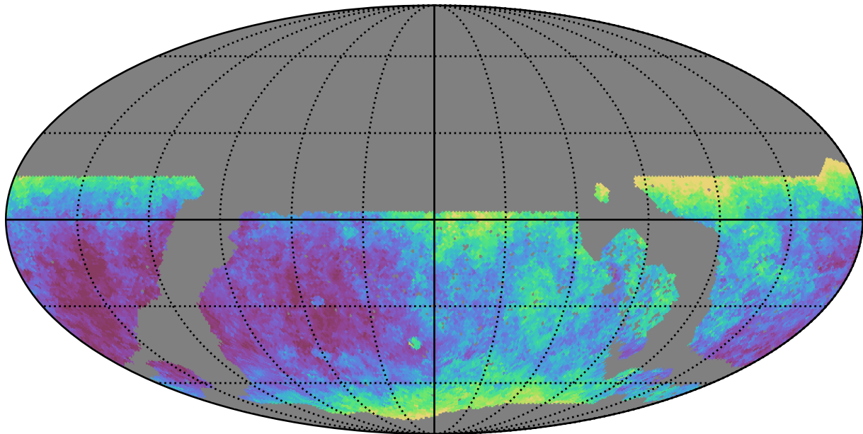
noroll_mjdp60_v3.4_10yrs WFD y band: Median seeingEff
