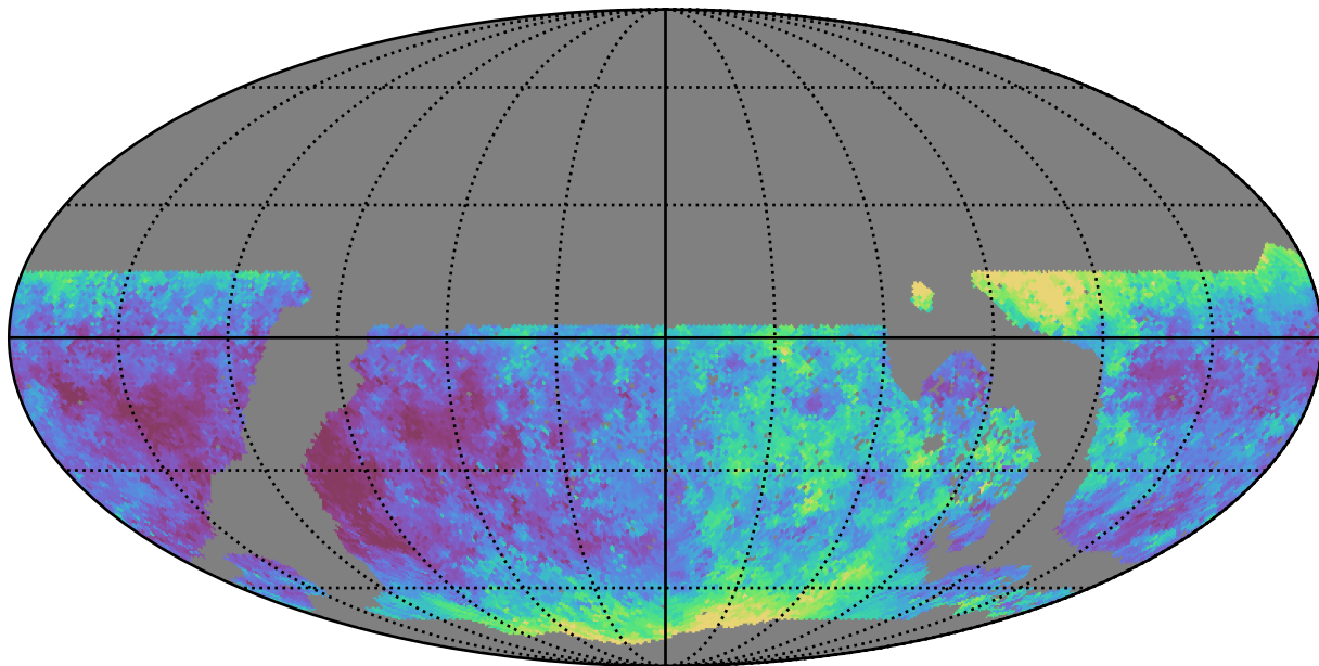
noroll_mjdp60_v3.4_10yrs WFD u band: Median seeingEff
