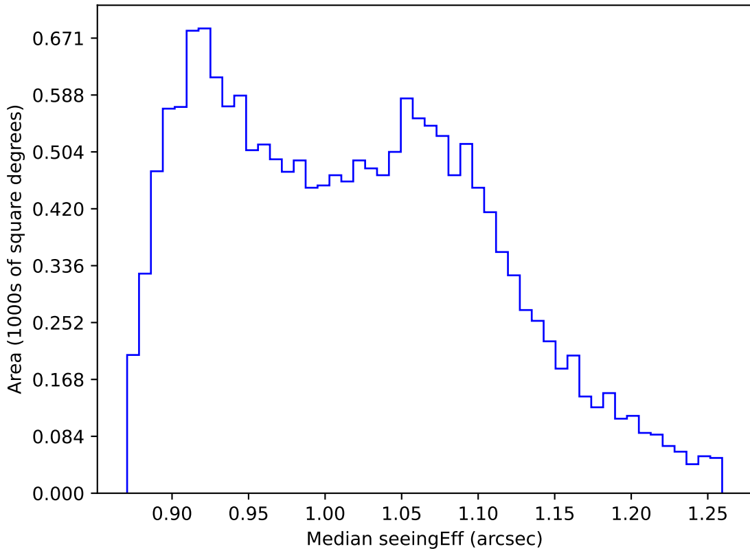
noroll_mjdp60_v3.4_10yrs WFD r band: Median seeingEff
