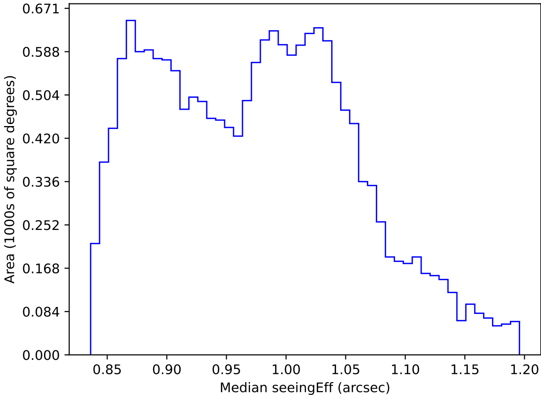
noroll_mjdp60_v3.4_10yrs WFD i band: Median seeingEff
