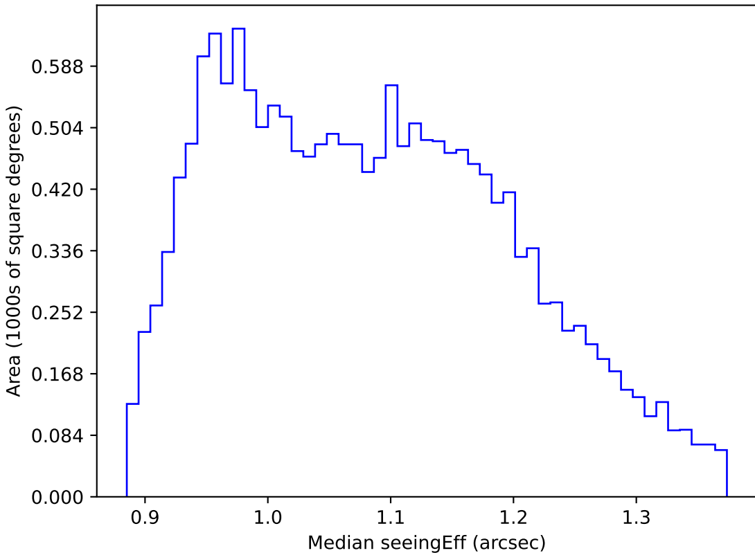
noroll_mjdp60_v3.4_10yrs WFD g band: Median seeingEff
