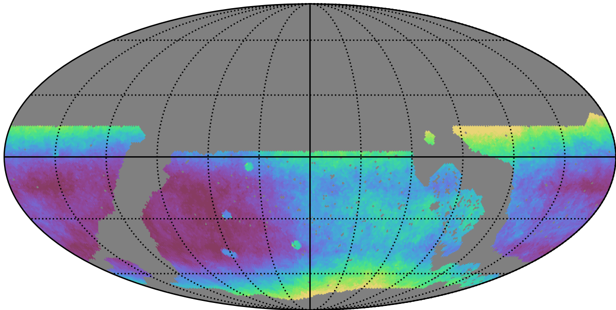
noroll_mjdp60_v3.4_10yrs WFD all bands: Median seeingEff
