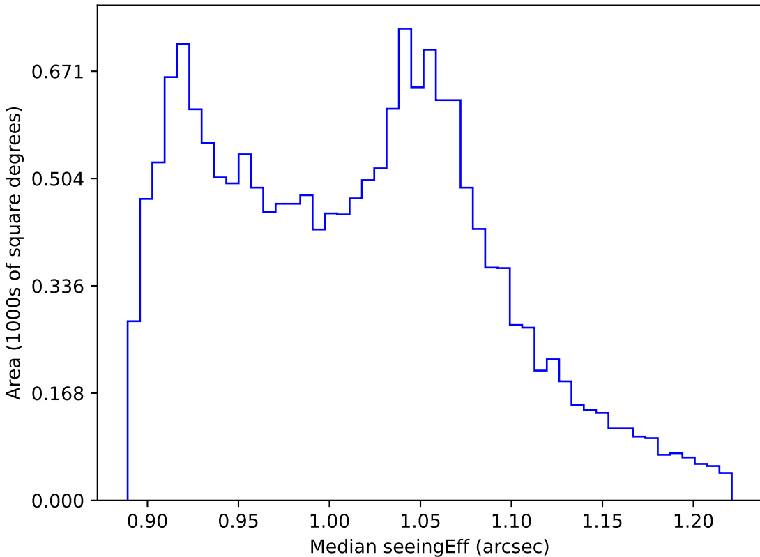
noroll_mjdp60_v3.4_10yrs WFD all bands: Median seeingEff
