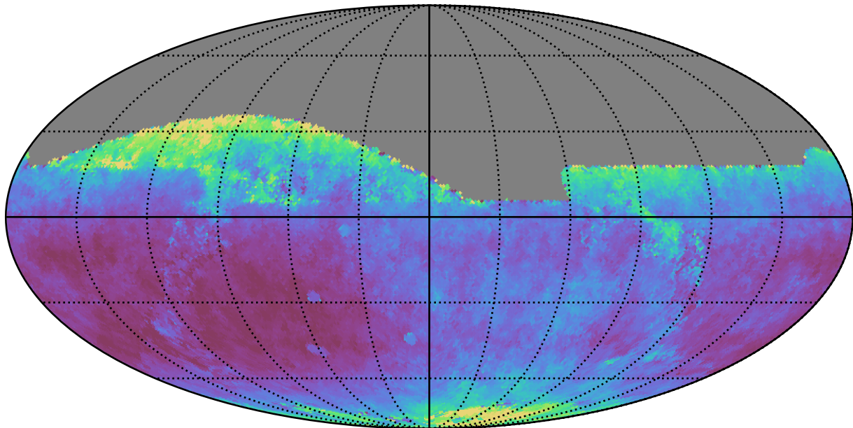
noroll_mjdp60_v3.4_10yrs All sky z band: Median seeingEff
