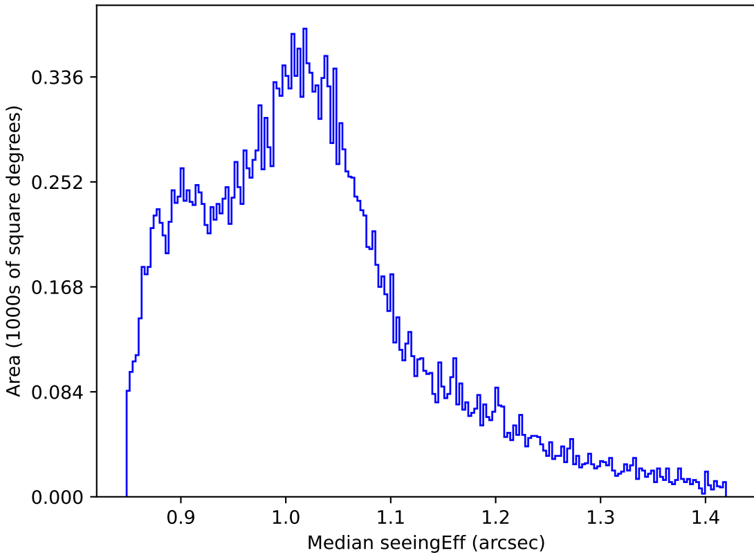
noroll_mjdp60_v3.4_10yrs All sky z band: Median seeingEff
