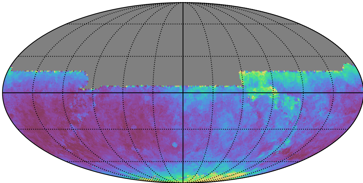
noroll_mjdp60_v3.4_10yrs All sky y band: Median seeingEff
