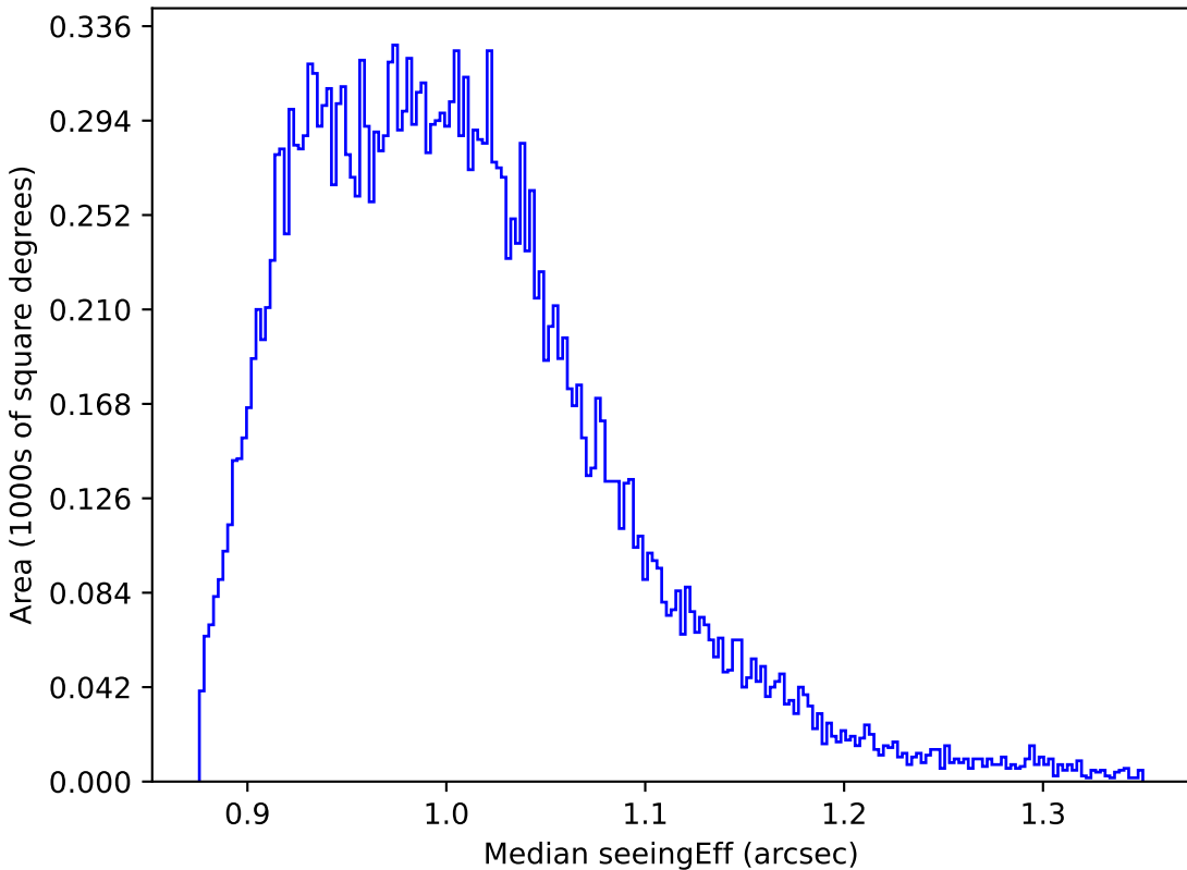
noroll_mjdp60_v3.4_10yrs All sky y band: Median seeingEff
