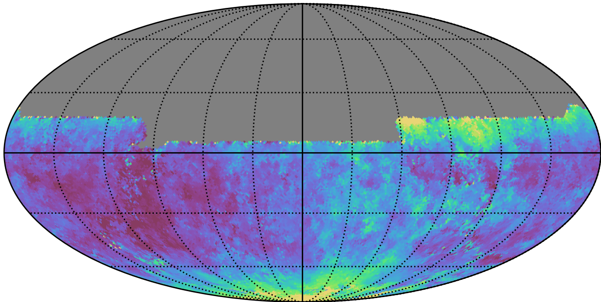
noroll_mjdp60_v3.4_10yrs All sky u band: Median seeingEff
