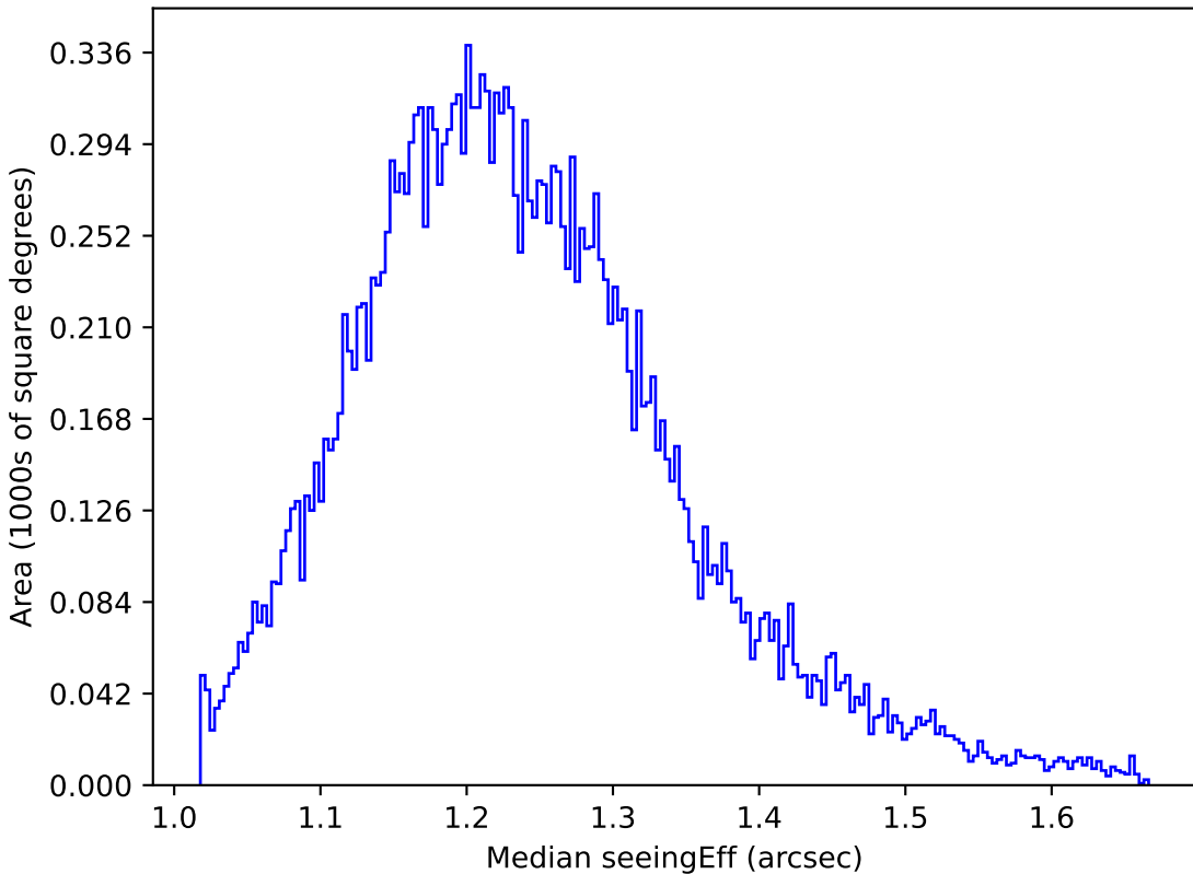
noroll_mjdp60_v3.4_10yrs All sky u band: Median seeingEff
