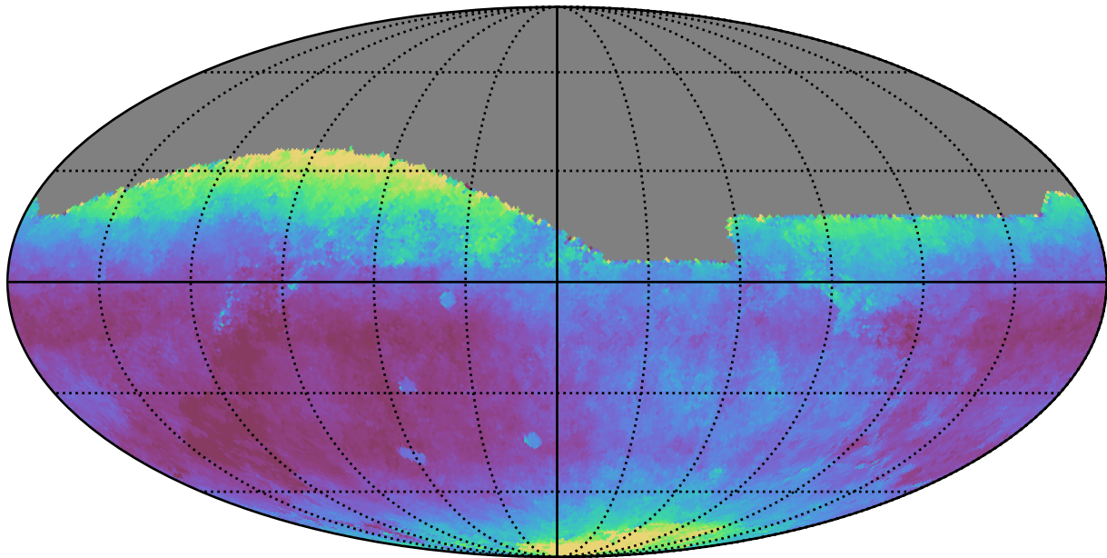
noroll_mjdp60_v3.4_10yrs All sky r band: Median seeingEff
