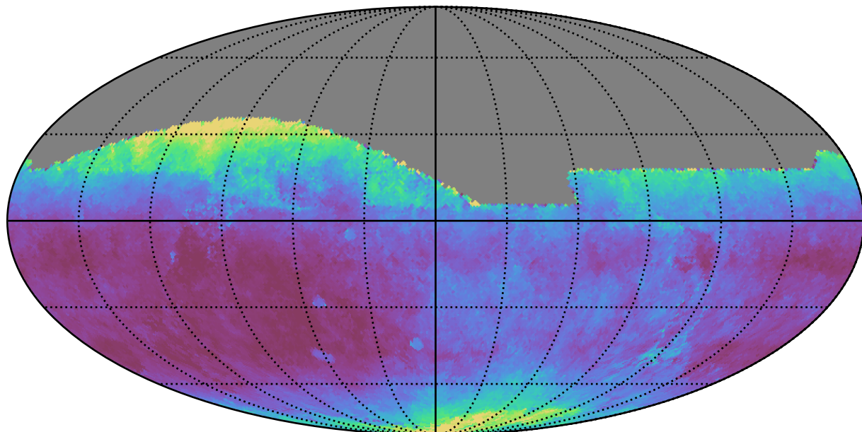
noroll_mjdp60_v3.4_10yrs All sky i band: Median seeingEff
