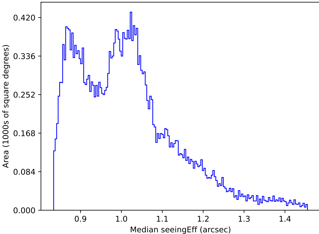
noroll_mjdp60_v3.4_10yrs All sky i band: Median seeingEff
