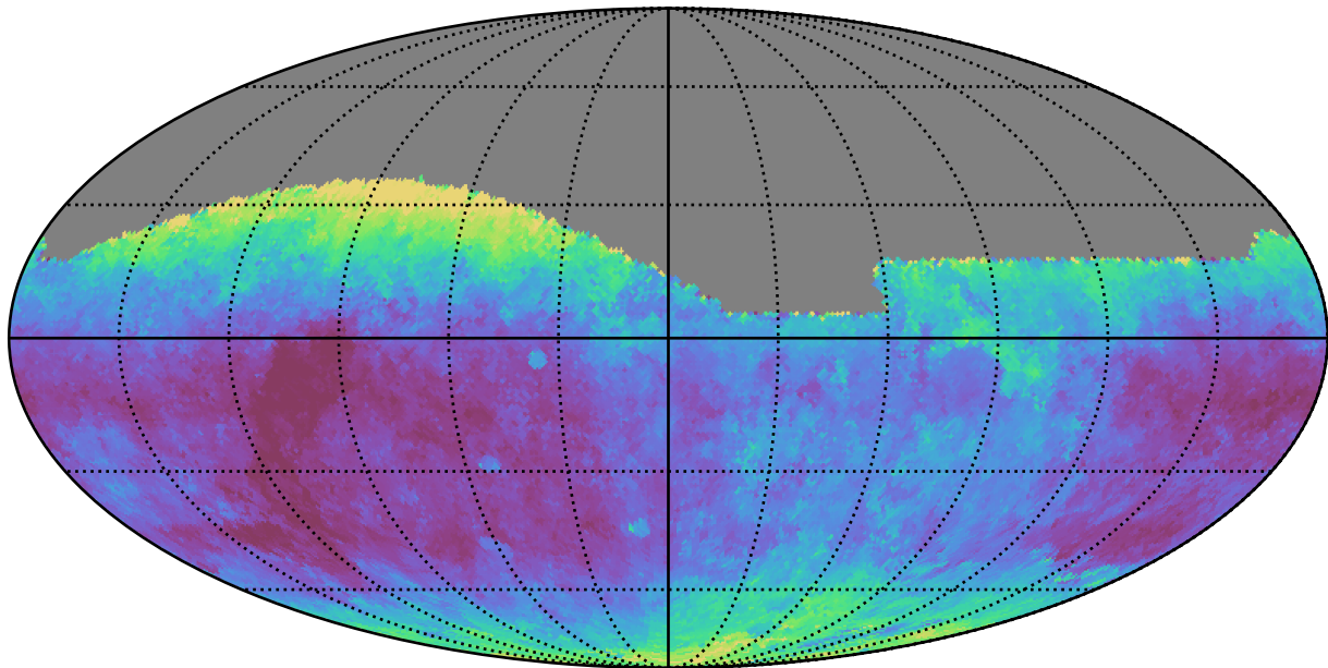
noroll_mjdp60_v3.4_10yrs All sky g band: Median seeingEff
