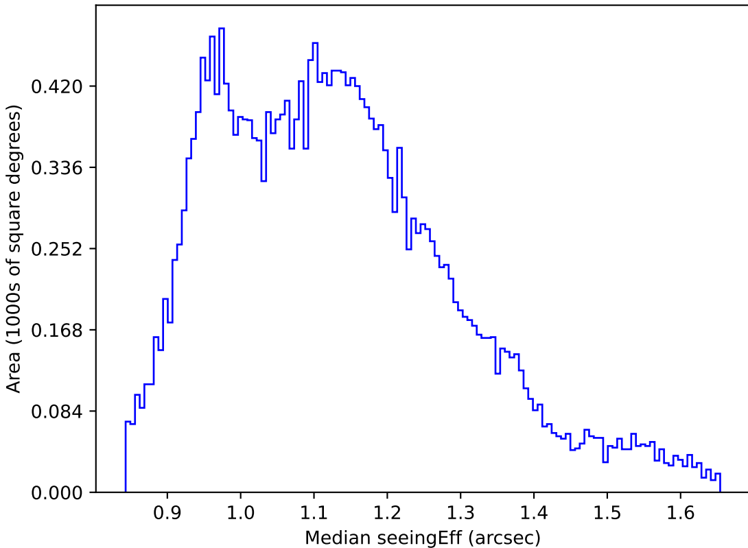
noroll_mjdp60_v3.4_10yrs All sky g band: Median seeingEff
