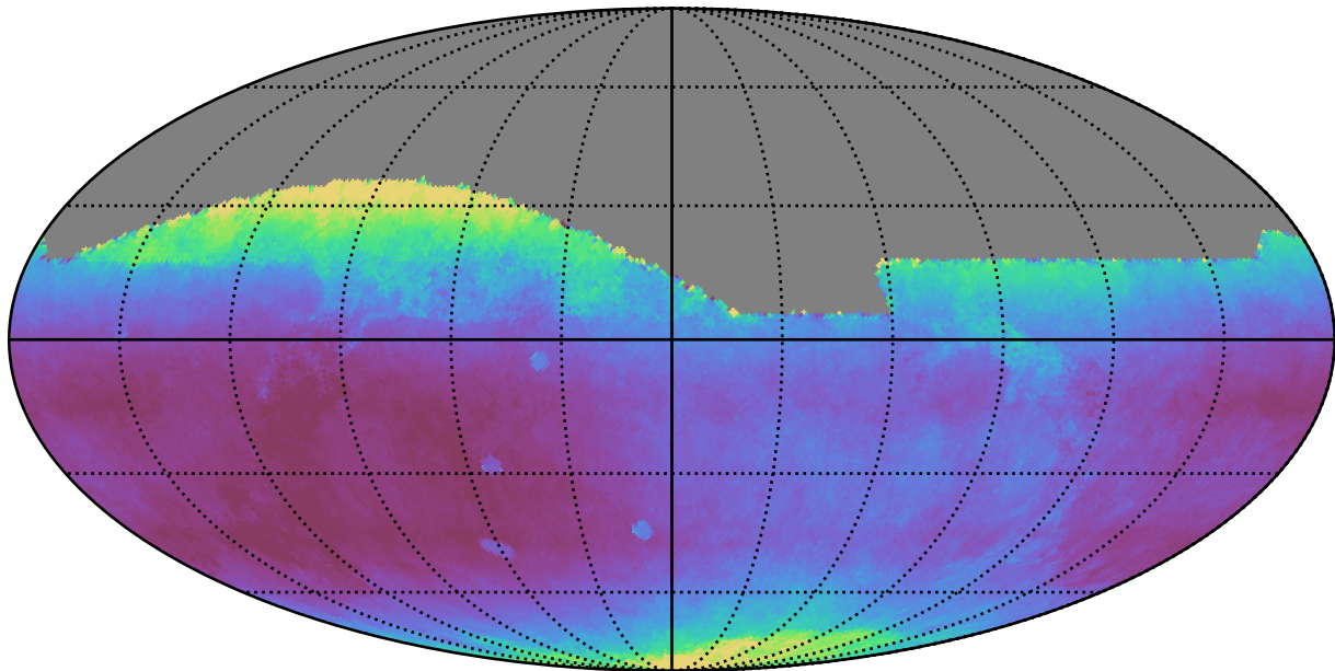
noroll_mjdp60_v3.4_10yrs All sky all bands: Median seeingEff
