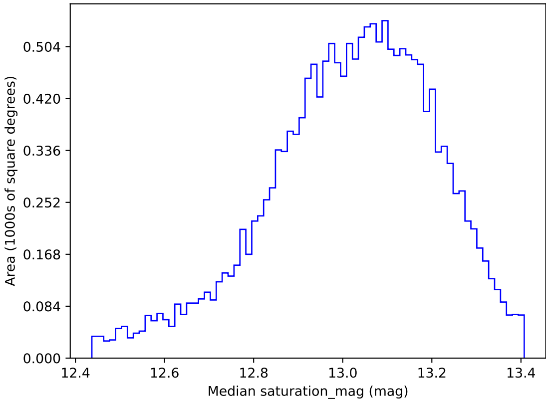
noroll_mjdp60_v3.4_10yrs WFD u band: Median saturation_mag
