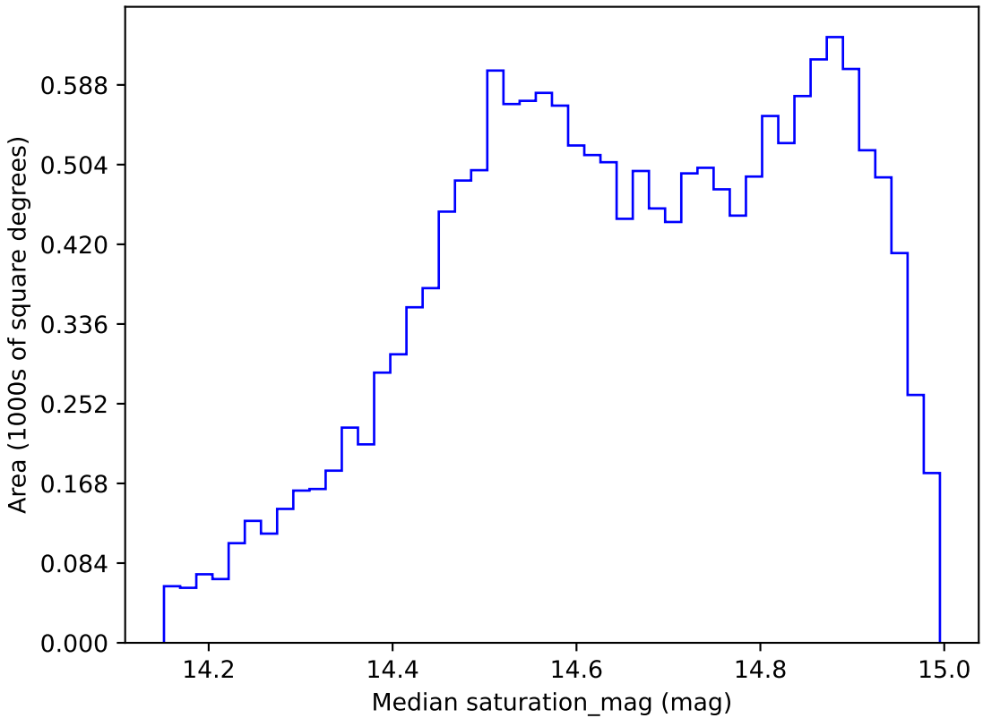
noroll_mjdp60_v3.4_10yrs WFD r band: Median saturation_mag
