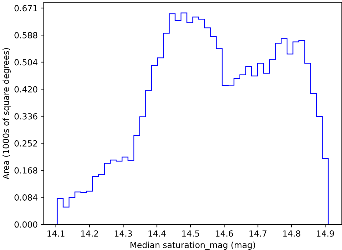
noroll_mjdp60_v3.4_10yrs WFD i band: Median saturation_mag
