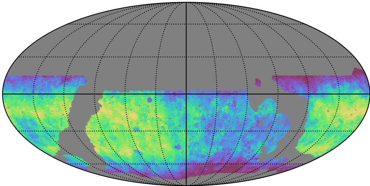
noroll_mjdp60_v3.4_10yrs WFD g band: Median saturation_mag
