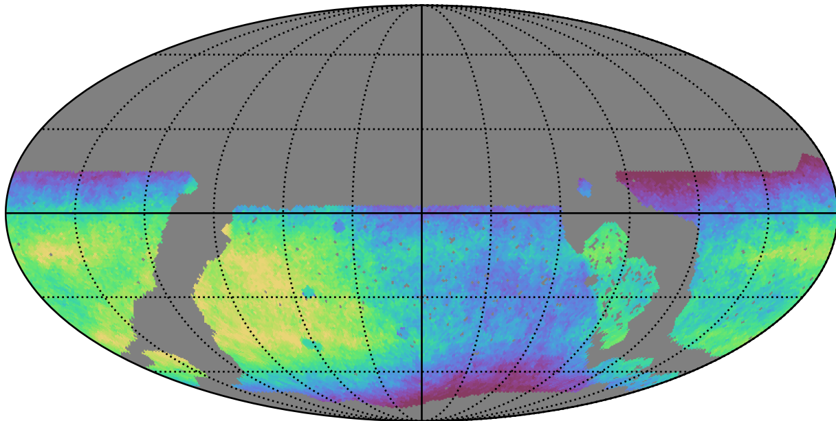
noroll_mjdp60_v3.4_10yrs WFD all bands: Median saturation_mag
