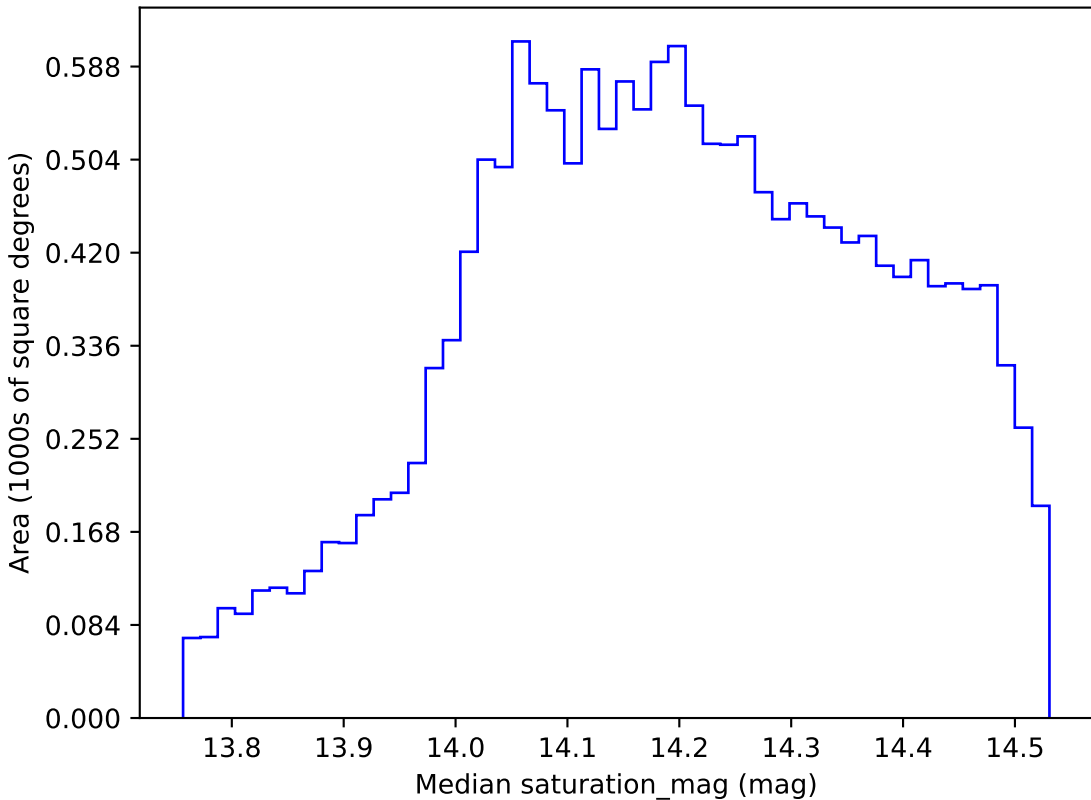
noroll_mjdp60_v3.4_10yrs WFD all bands: Median saturation_mag
