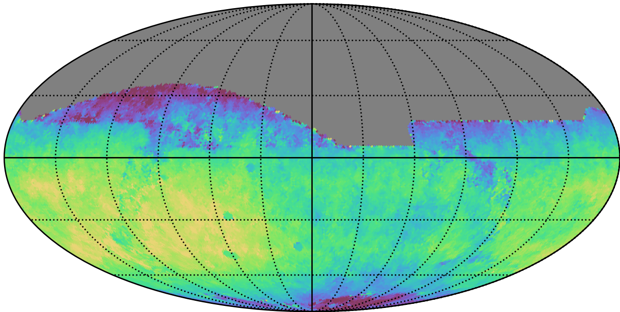
noroll_mjdp60_v3.4_10yrs All sky z band: Median saturation_mag
