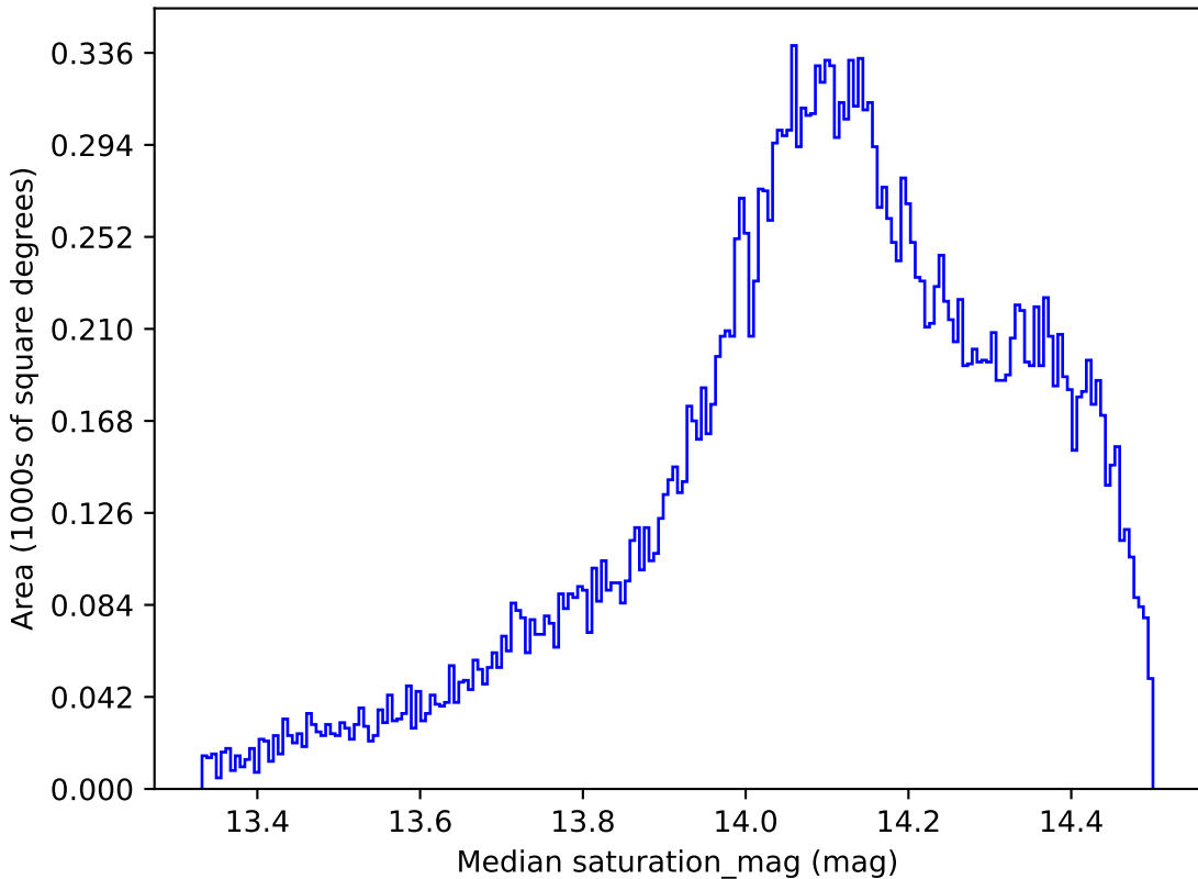
noroll_mjdp60_v3.4_10yrs All sky z band: Median saturation_mag
